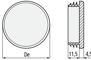
Tube dimensions
